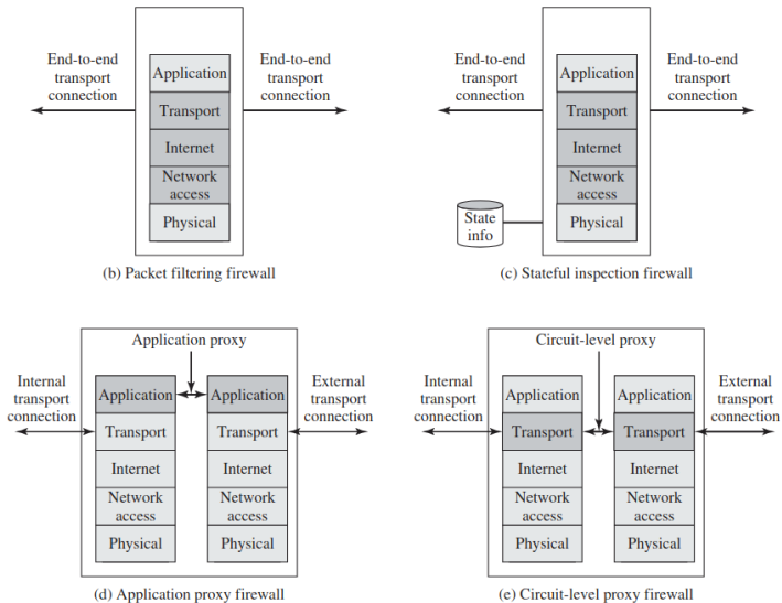
Figure 9.1 Types of Firewalls
