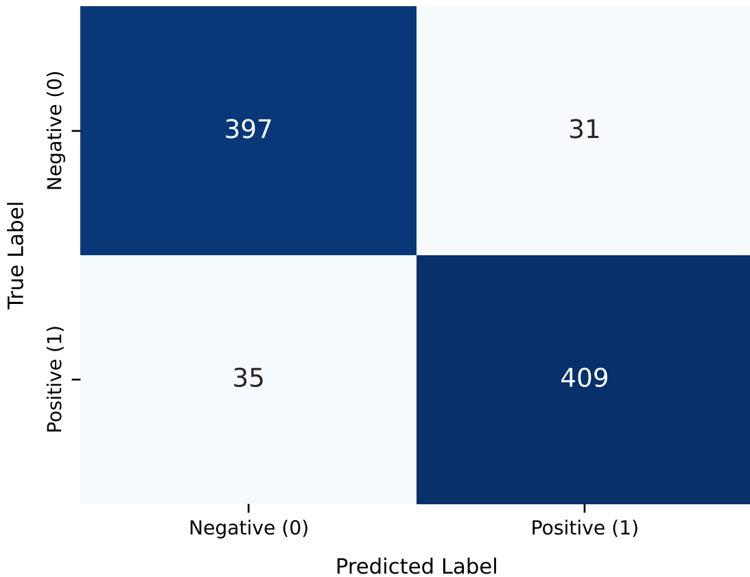
Confusion Matrix - BERT (SST-2)
