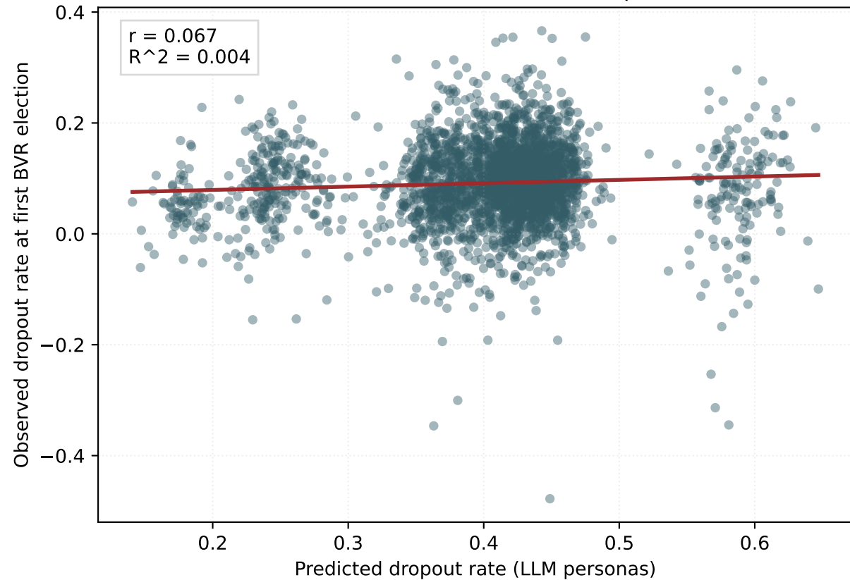
Predicted vs observed BVR dropout
