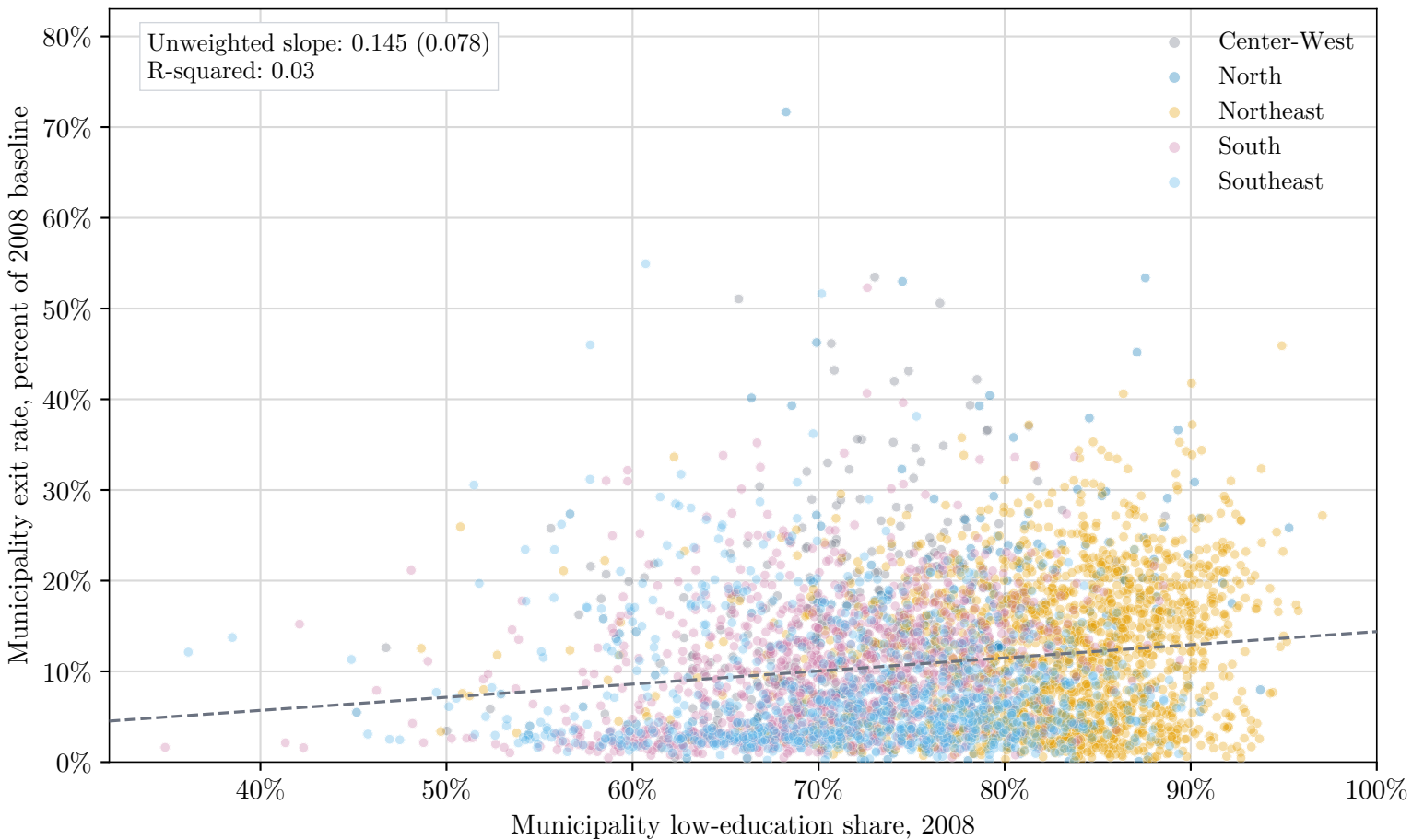
Municipal exit rates track baseline low-education shares
