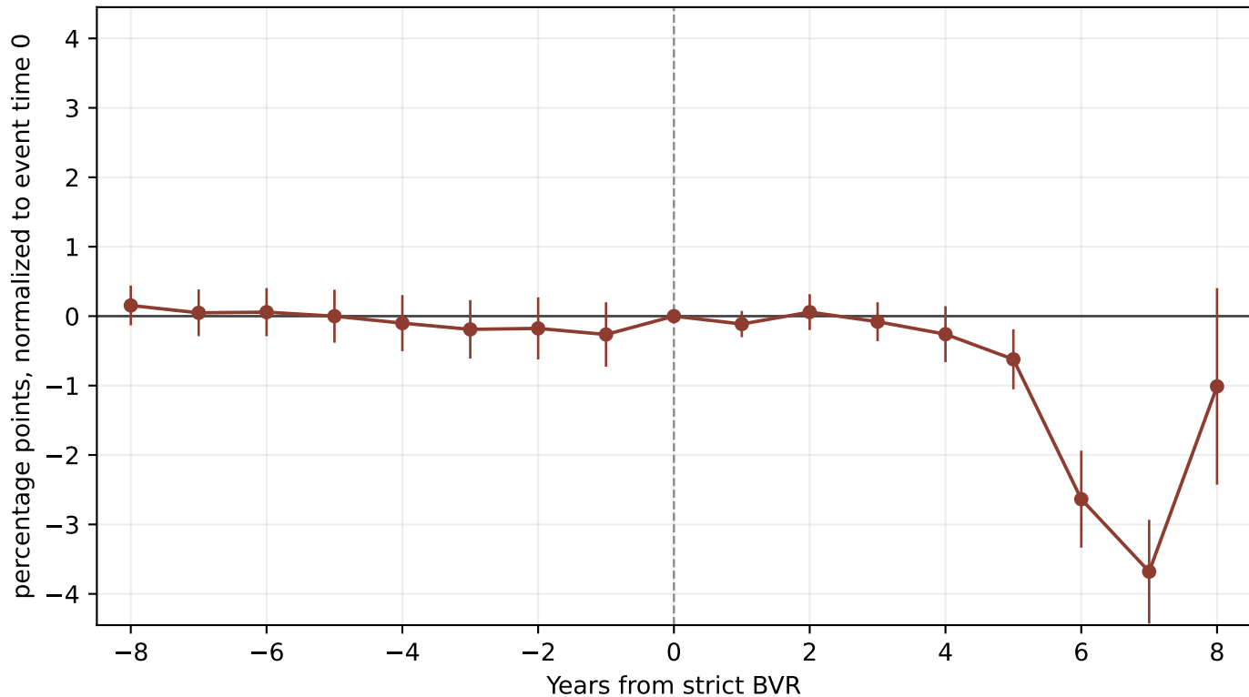
Municipal Taxa Abandono Ef Anos Finais post mean e1..e8=-1.04, pre=pass
