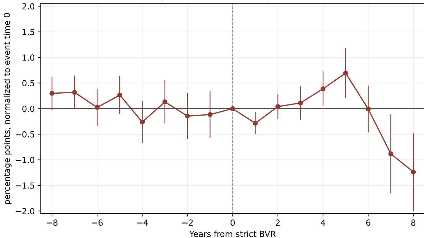
Total Taxa Repetencia Em post mean e1..e8=-0.147, pre=pass
