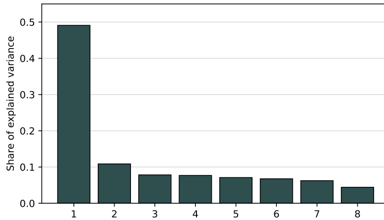
Figure 32: Trust Index: Share of Explained Variance by Principal Component
