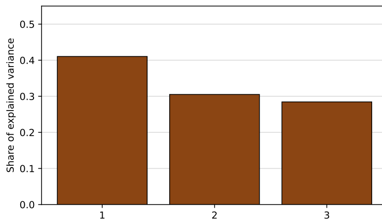
Figure 33: Democracy Index: Share of Explained Variance by Principal Component
