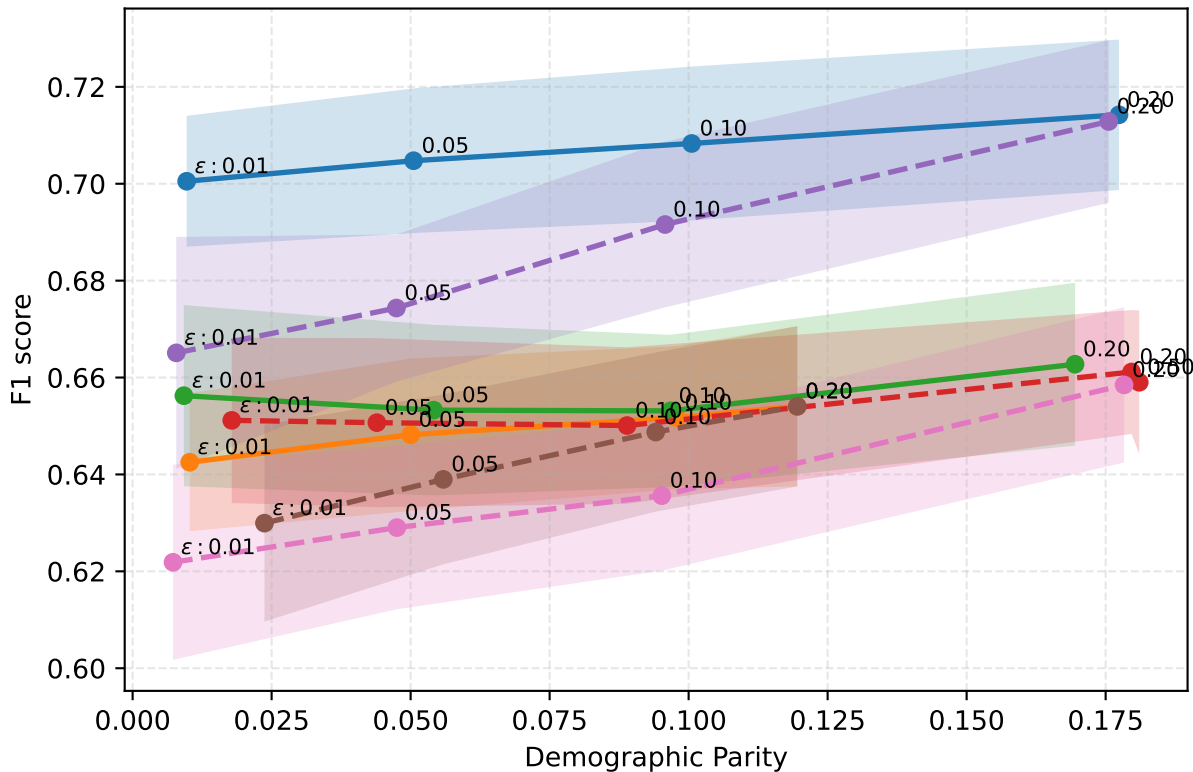
Fairness-Accuracy Trade-off
