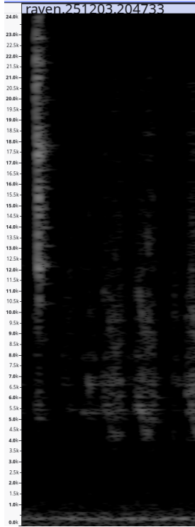
Fig. 2. Spectrogram of a single courtship chirp, which spans from 5kHz to 24 kHz frequency range.
