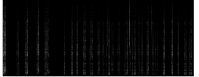
Fig. 1. A clip showing different cricket chirps. Short courtship chirps at higher frequencies, with other cricket chirps appearing across the whole frequency range.
