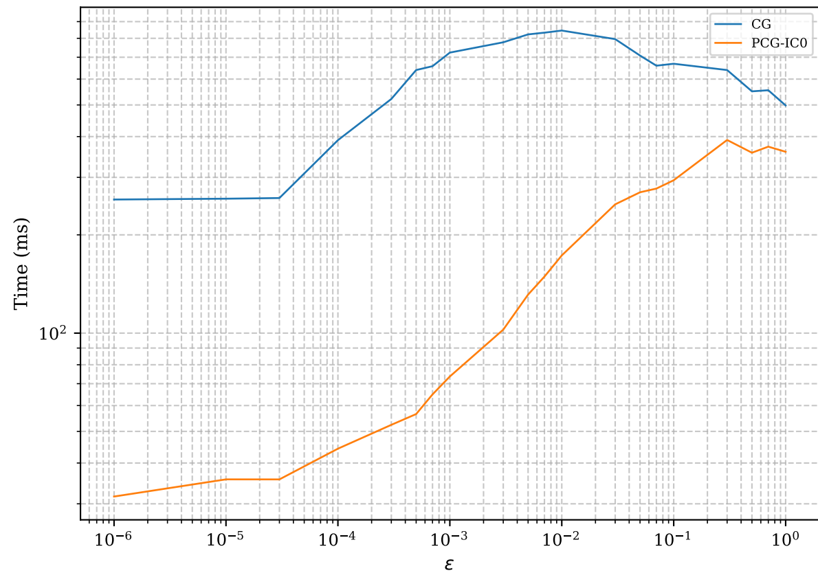
Solving time (ms) vs. \varepsilon for N = 128
