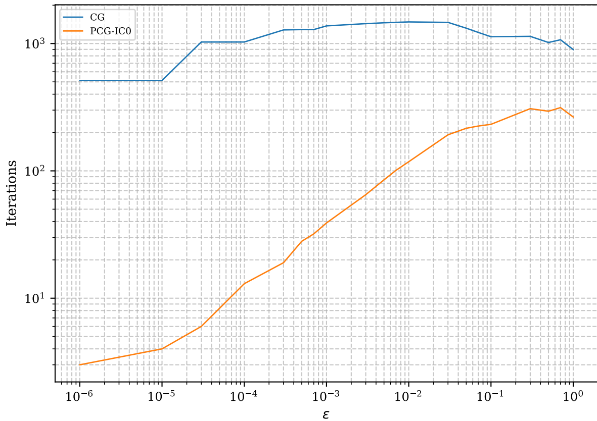
Iterations vs. \varepsilon for N = 512
