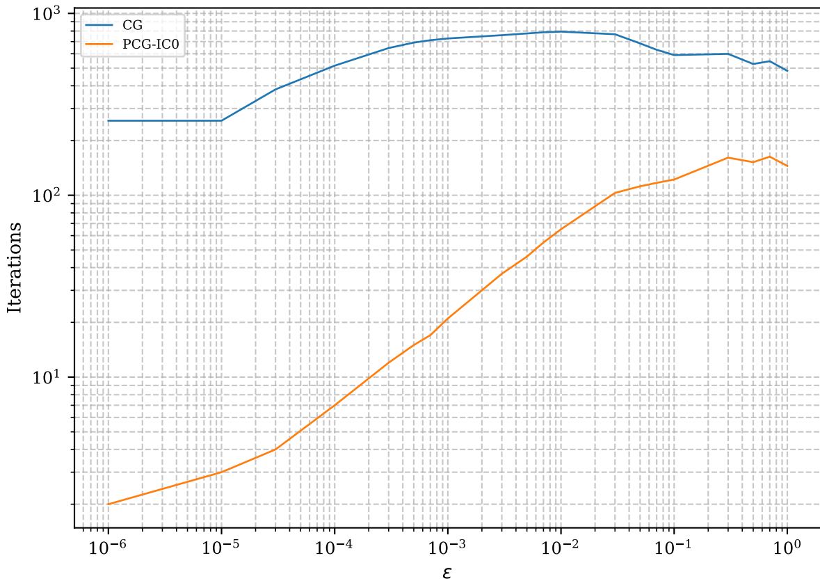
Iterations vs. \varepsilon for N = 256
