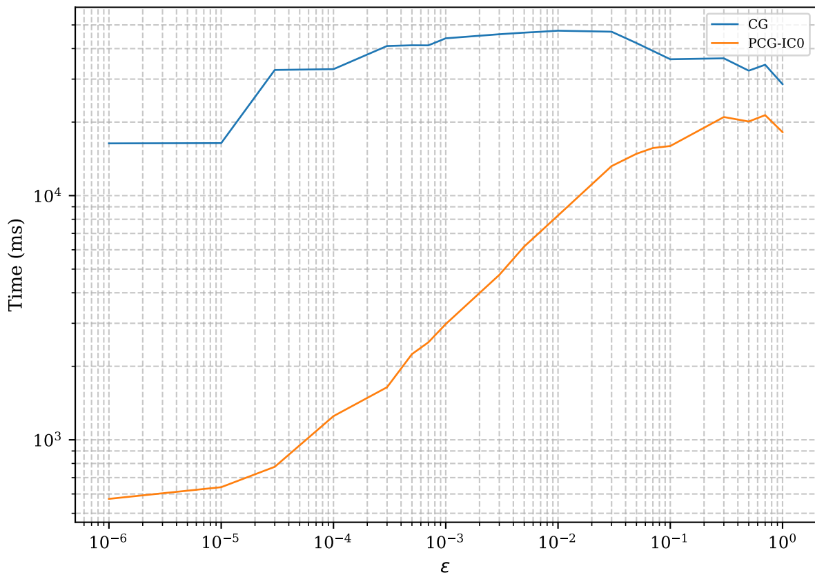
Solving time (ms) vs. \varepsilon for N = 512
