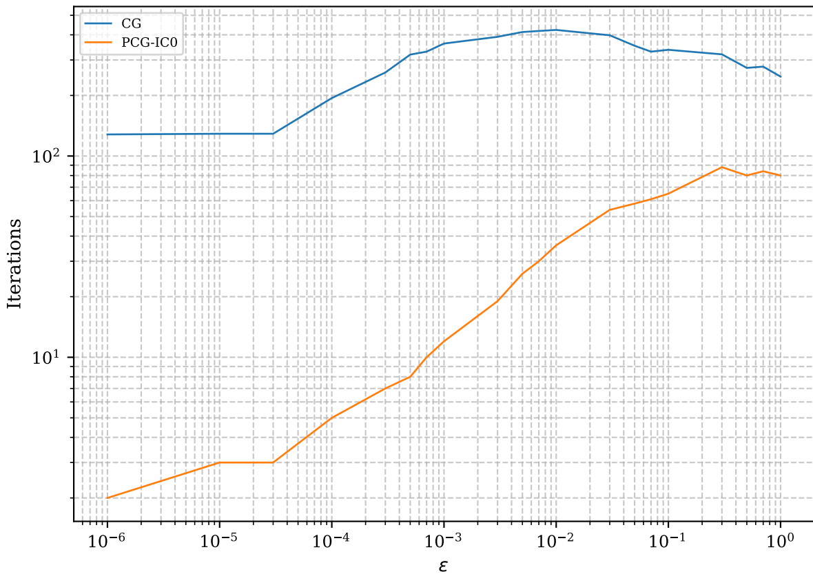
Iterations vs. \varepsilon for N = 128
