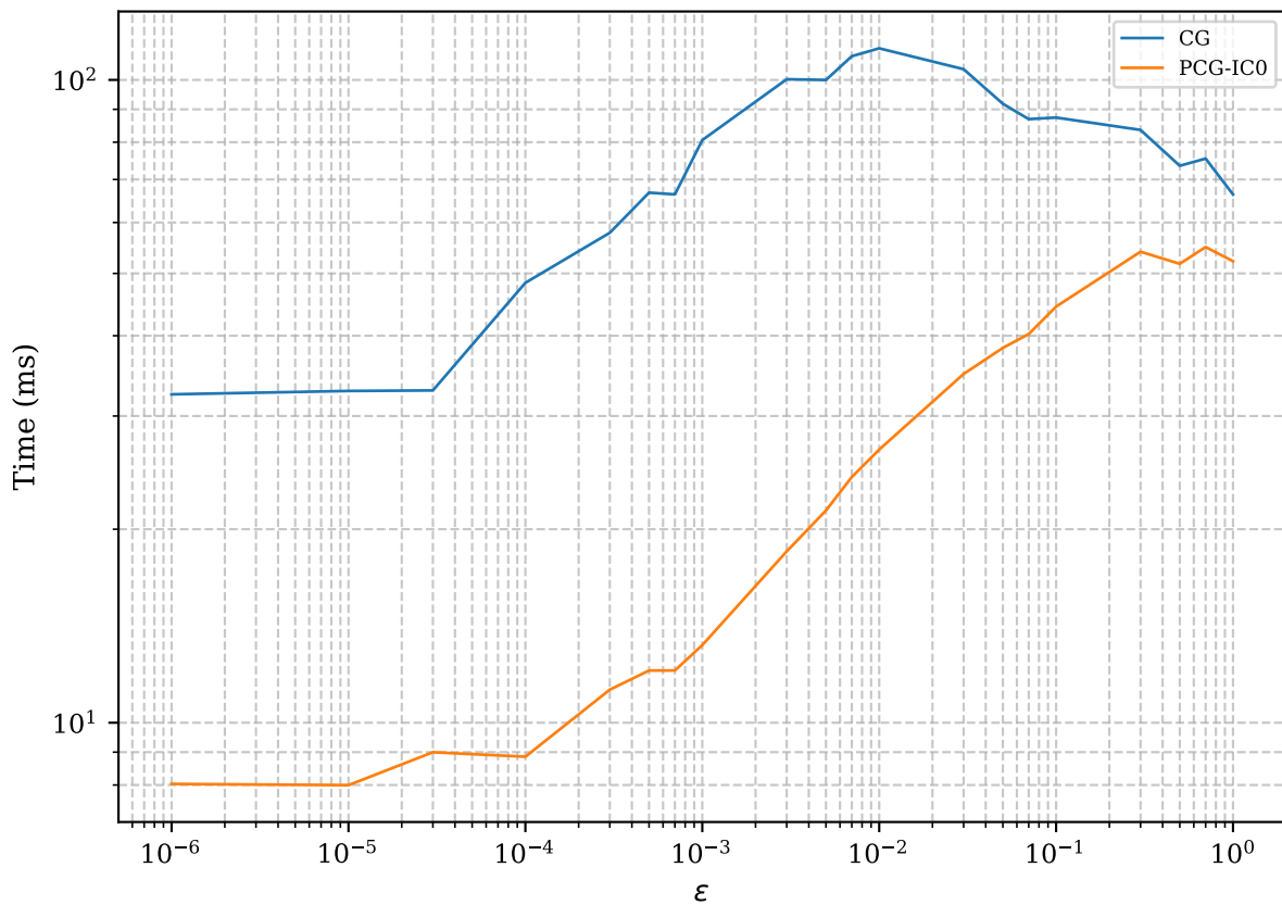
Solving time (ms) vs. \varepsilon for N = 64
