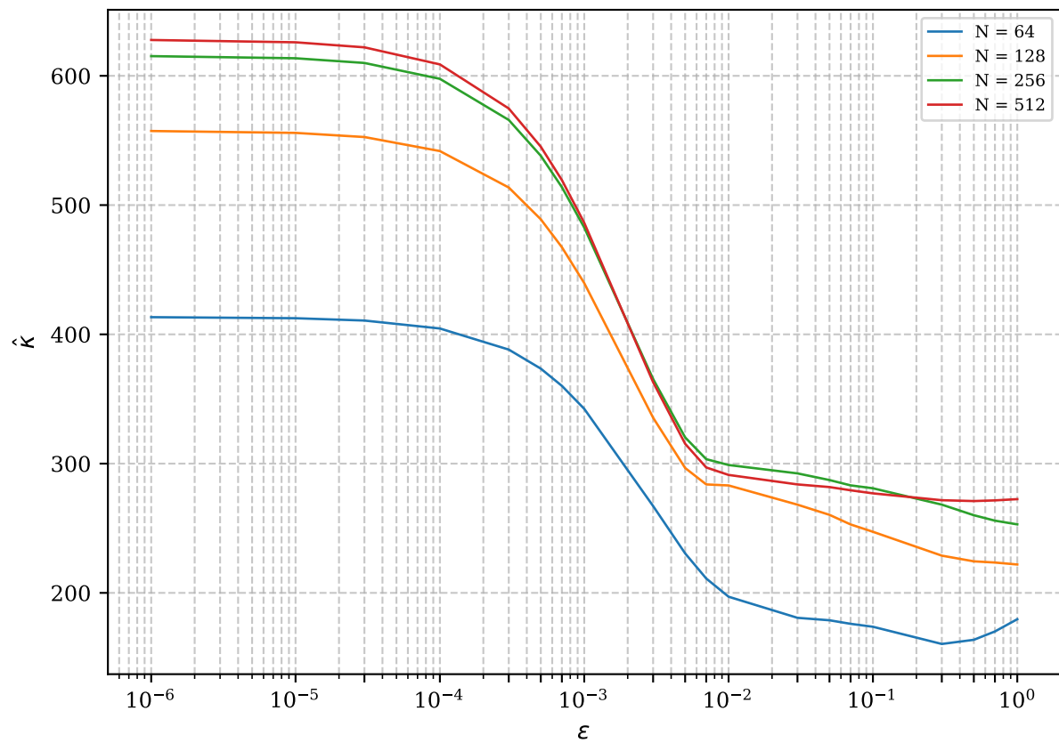
\hat{\kappa} vs. \varepsilon for CG
