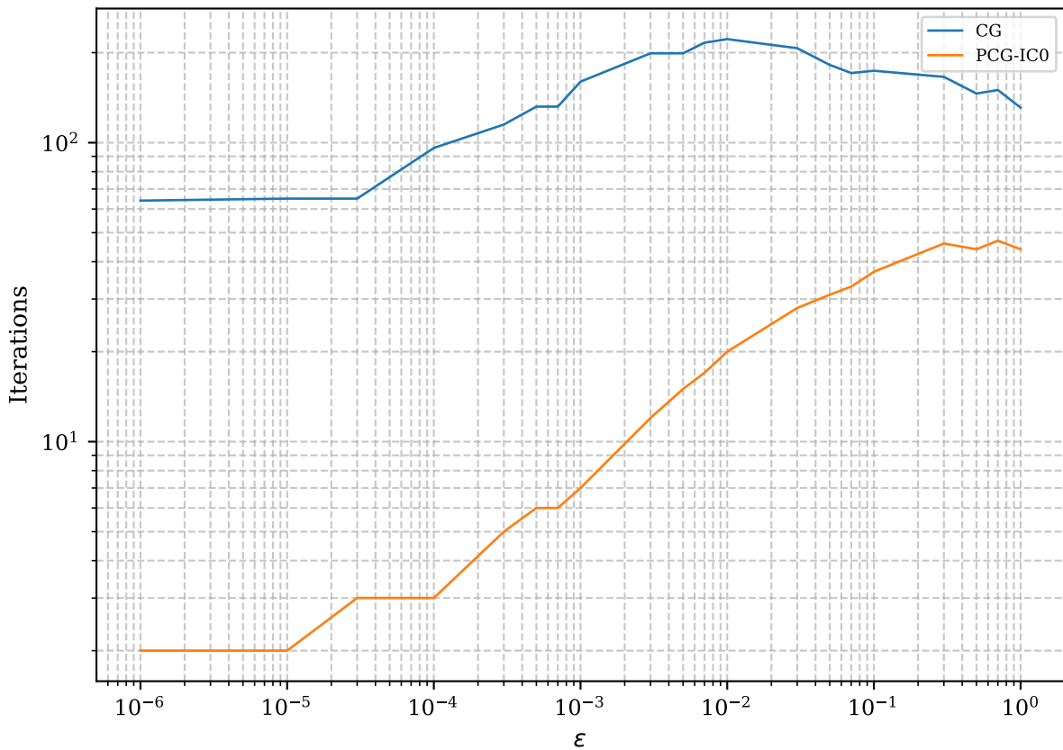
Iterations vs. \varepsilon for N = 64
