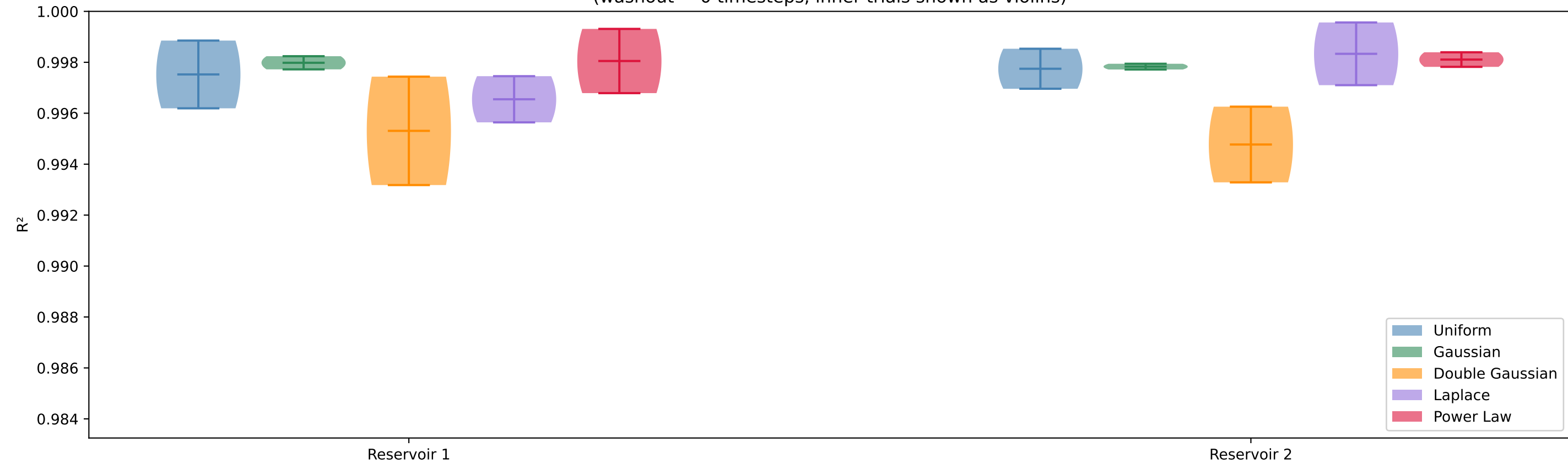
SC1 Fixed-Reservoir — R^2 per reservoir and read-in distribution (washout = 0 timesteps, inner trials shown as violins)
