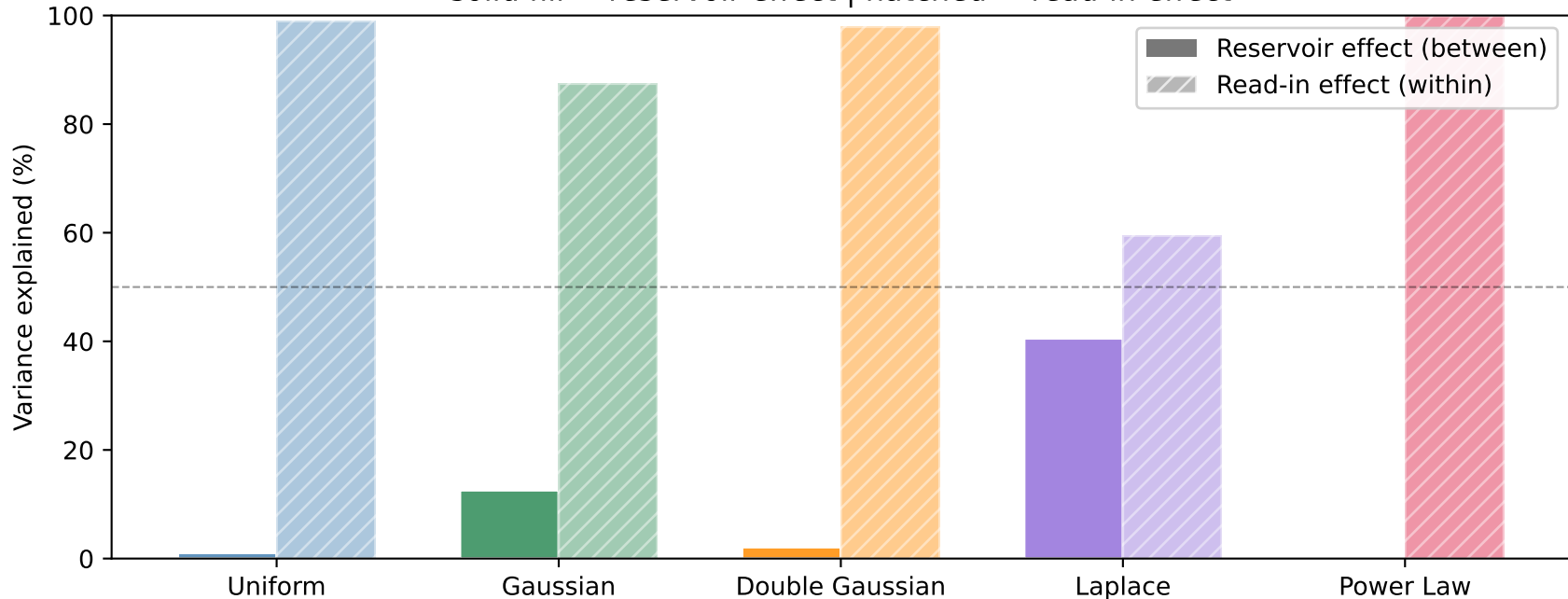
SC1 Fixed-Reservoir — Variance decomposition: reservoir vs. read-in weights solid fill = reservoir effect | hatched = read-in effect
