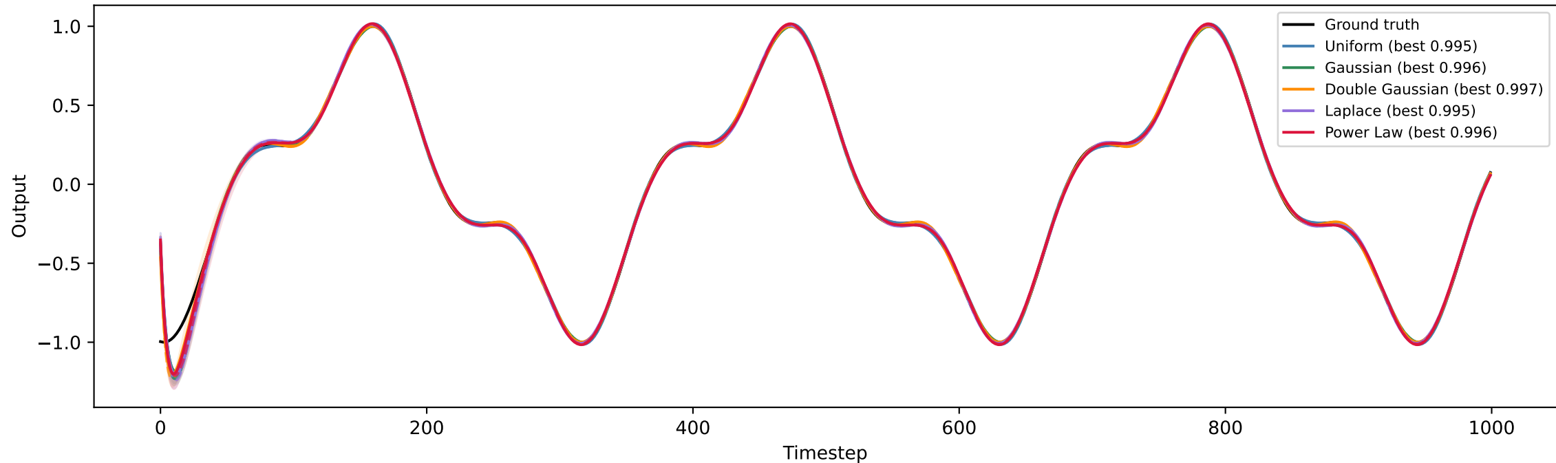
SC1 Fixed Read-In | Best predictions per distribution
