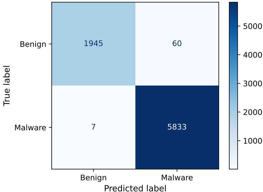
RF Confusion Matrix
