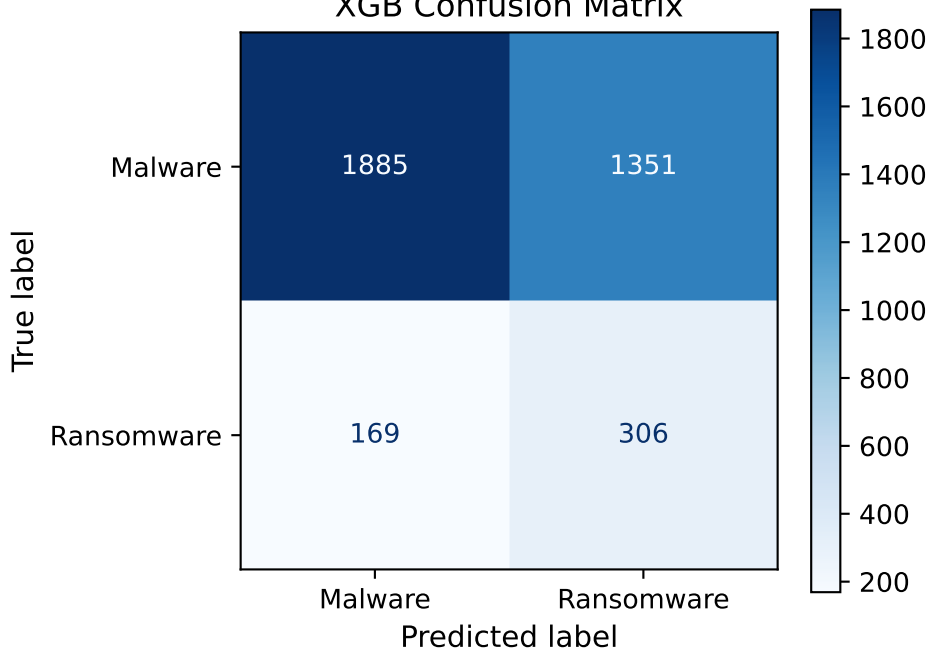
XGB Confusion Matrix
