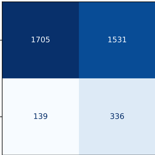
SVM Confusion Matrix
