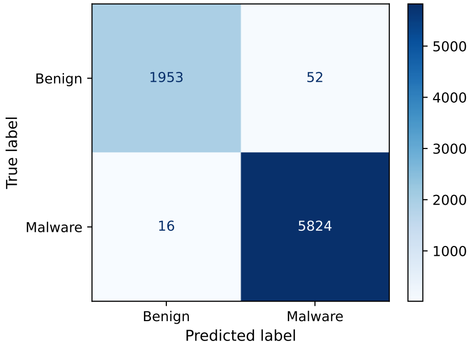
XGB Confusion Matrix
