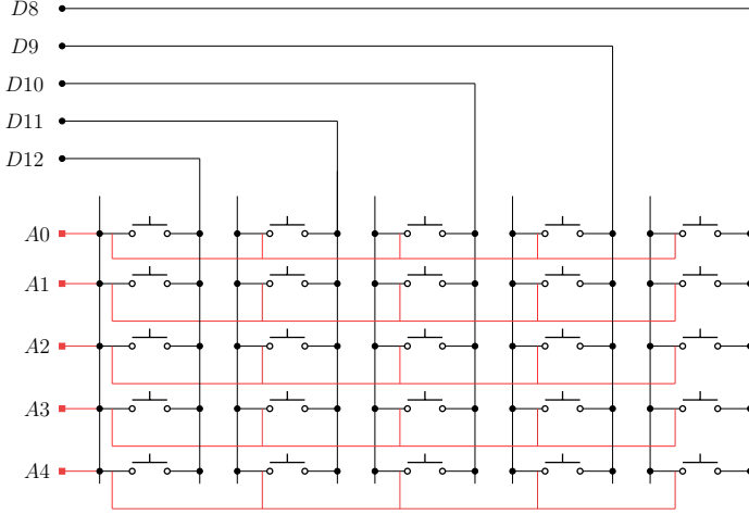
Fig. 1. Button Matrix
