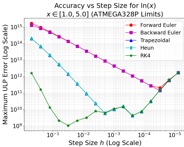
Fig. 4. Accuracy versus step size
