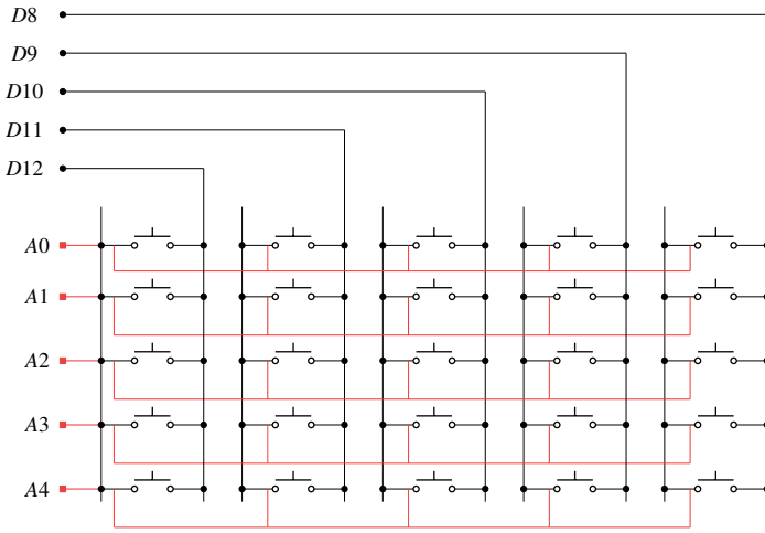
Fig. 1: Button Matrix
