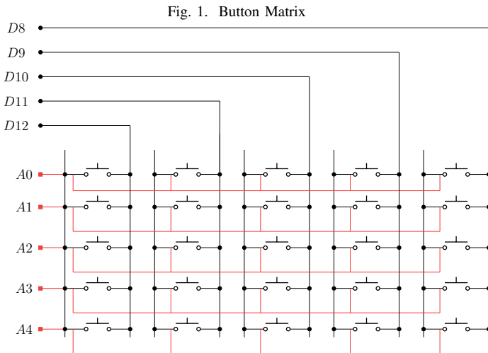
Fig. 1. Button Matrix
