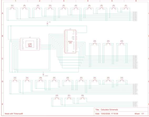
Fig. 2: Schematic of Circuit.
