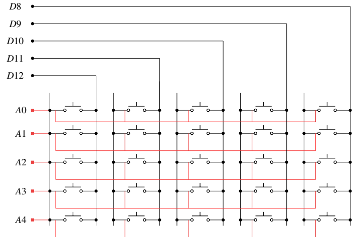
Fig. 1: Button Matrix
