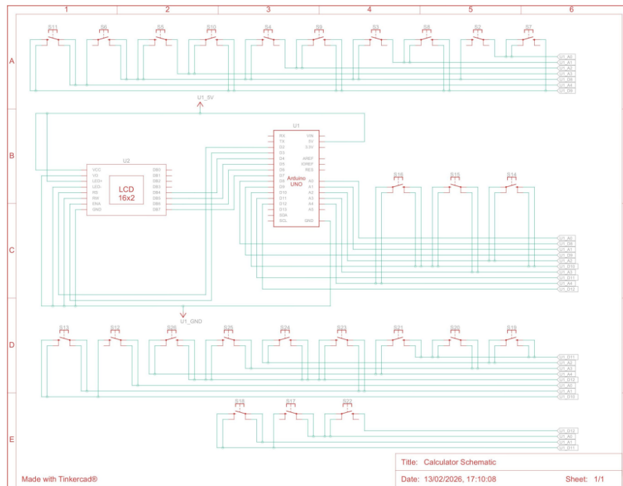
Fig. 1: Schematic of Scientific Calculator
