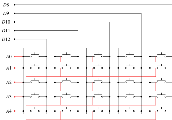
Fig. 2: Button Matrix
