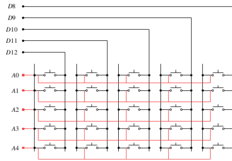
Fig. 2: Button Matrix
