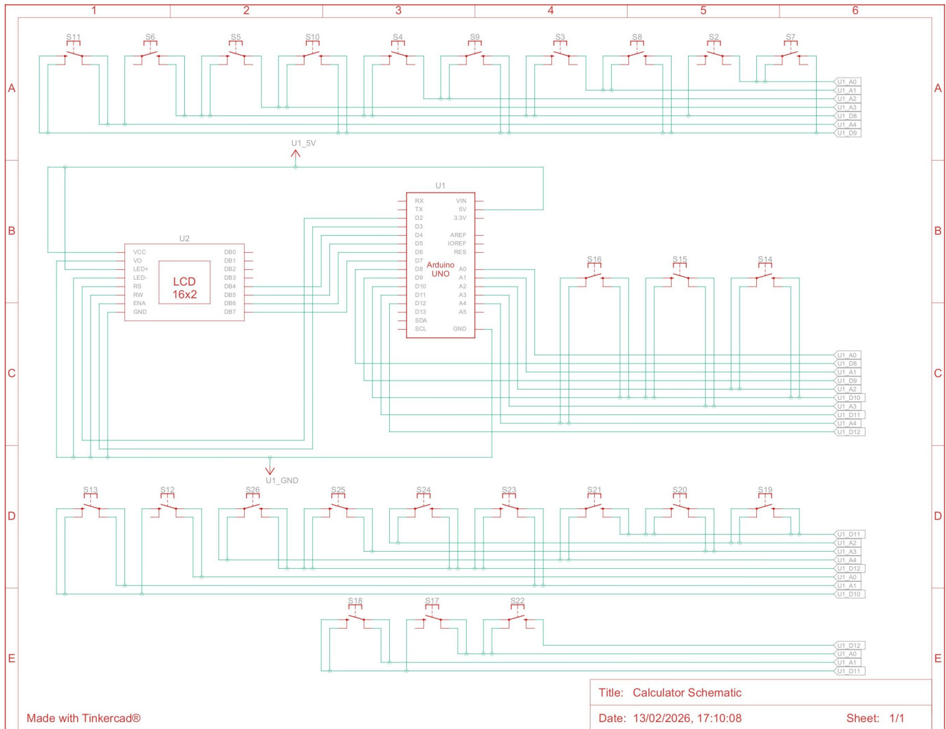
Fig. 1: Schematic of Scientific Calculator
