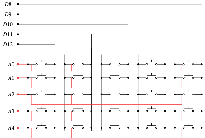
Fig. 1: Button Matrix
