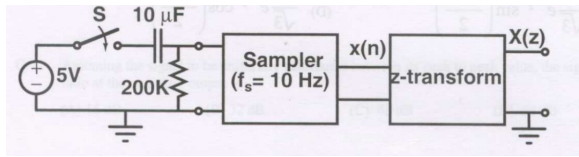
Fig. 1.2.92.1: Circuit
