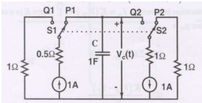
Fig. 1.1.86.1: Circuit
