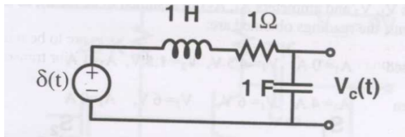
Fig. 98.1: Circuit
