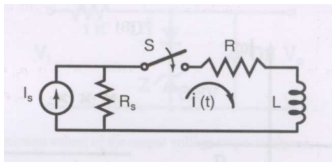
Fig. 1.1.81.1: Circuit
