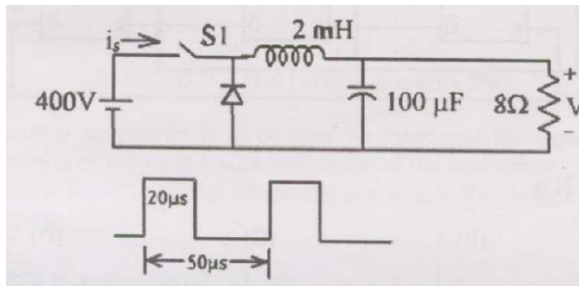
Fig. 1.1.69.1: Circuit
