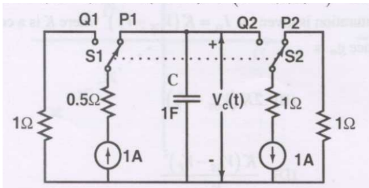
Fig. 1.1.86.1: Circuit
