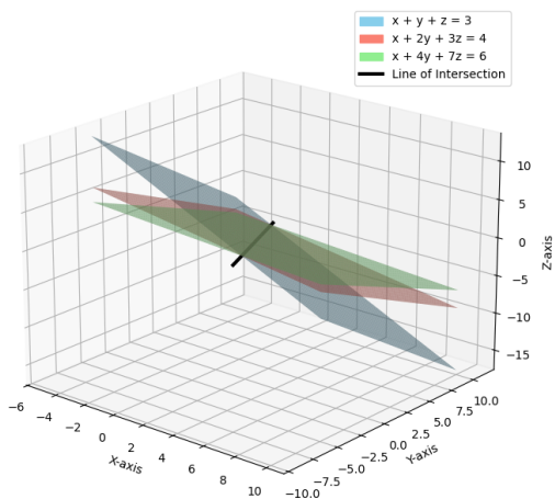
Intersection of Three Planes when k=7
