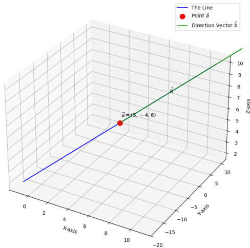
Vector Equation of the Line
