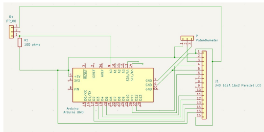
Fig. 2: Circuit Schematic of the simple voltage divider (Setup 2)
