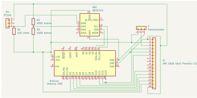
Fig. 3: Circuit Schematic of the High-Precision Wheatstone Bridge
