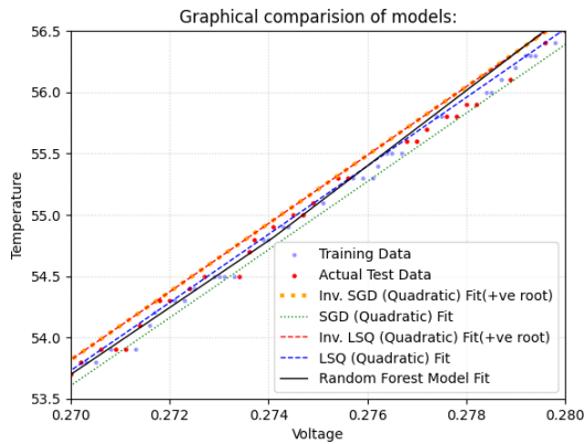
Fig. 4: Comparison of Random Forest, Inverse LSQ, LSQ, SGD and Inverse SGD Regressor predictions against actual test data for the Wheatstone bridge with ADC for temperatures between 53.5°C to 56.5°C
