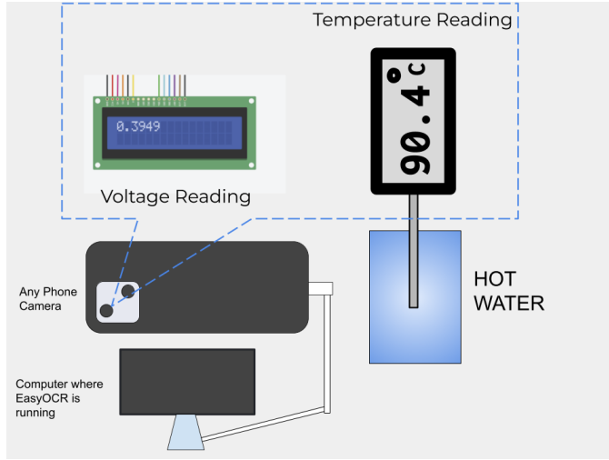
Fig. 3: Auto-Trainer representation
