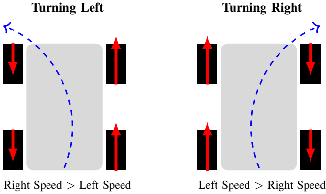
Fig. 6: Skid Steering Visualization
