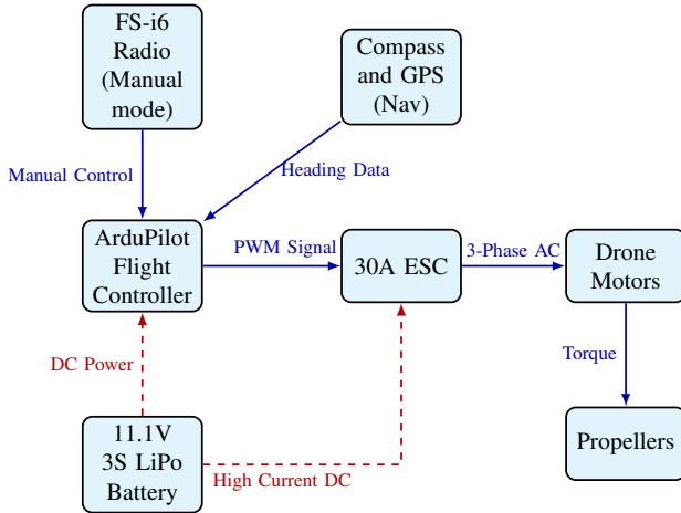
Fig. 1: Original Drone Architecture
