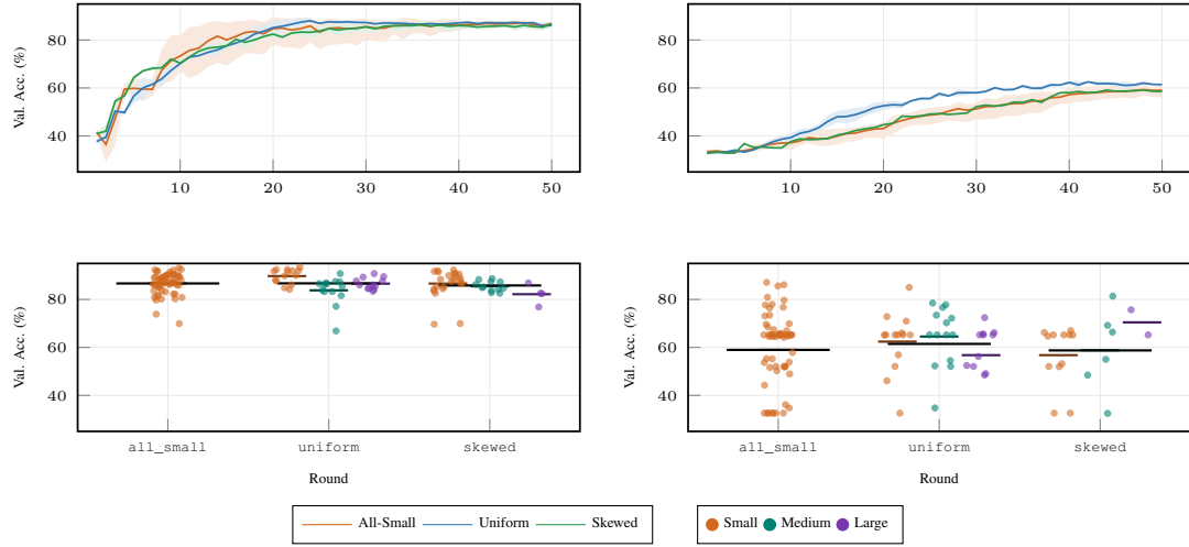
Fig. 8. FedMD tier-heterogeneity ablation on HomeOccupancy. Top: mean validation-accuracy curves over completed seeds (shaded bands: seed range), IID (left) and non-IID (right) on a shared y-axis. Bottom: per-client final accuracy (mean of the last five rounds, seeds pooled). Each distribution column is subdivided by architecture tier—small (orange), medium (teal), large (purple)—so tier counts are visible (e.g. skewed : 12/6/2); short coloured dashes mark tier means, the long black dash the column mean. Tier means differ by only a few points within every setting: under soft-label sharing, per-client accuracy is governed by the data partition, not by model capacity.
