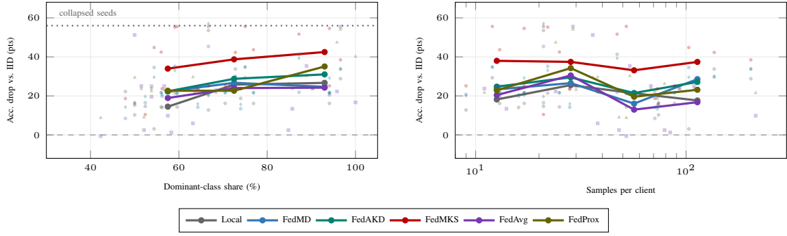
Fig. 8. Partition imbalance, not partition size, drives the per-client accuracy decline under non-IID (HomeOccupancy). Dots are individual clients; thick lines are binned means. The y-axis is the drop from the method’s own IID mean. (a) The decline grows steadily with the dominant-class share for every method that keeps per-client models—e.g. FedAvg in its surviving seed falls from \approx 0 to \approx 24 points of drop across the share range ( r=+0.73 for FedProx)—while the collapsed FedAvg/FedProx seeds form a flat band at \approx 56 points (dotted): their bias is total and independent of the partition. (b) The same decline is uncorrelated with the number of samples a client holds ( r\approx 0 ): at this scale, balance matters and quantity does not.
