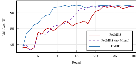
Fig. 10. FedMKS vs. FedDF validation accuracy on HomeOccupancy (IID, 30 rounds, 10 clients). The dashed curve is a FedMKS ablation with Mixup augmentation on the public set disabled.
