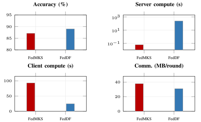
Fig. 11. Compute, communication, and accuracy comparison of FedMKS and FedDF on HomeOccupancy (cf. Table VII). FedMKS eliminates the server bottleneck at \approx 22\% higher communication and higher per-client compute.
