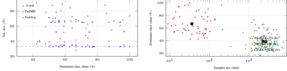
Fig. 7. Data distribution decides per-client accuracy. (a) HomeOccupancy non-IID: each client’s final accuracy vs. the dominant-class share of its Dirichlet partition. Local and FedMD accuracies degrade as the partition approaches a single class ( r=-0.36 for Local); FedAvg clients in the two collapsed seeds sit at chance at every share—collapse is a global property of the averaged model, not of any client’s data. (b) Per-client partitions of all benchmarks in the (samples, dominant-share) plane (all seeds pooled; large dots mark dataset means). HomeOccupancy occupies the high-skew/low-data corner—the regime where weight averaging can collapse—while MNIST and CIFAR-10 clients hold \approx 60\times more samples at lower dominant shares.
