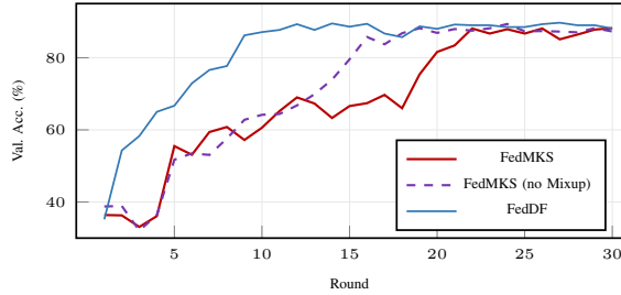
Fig. 9. FedMKS vs. FedDF validation accuracy on HomeOccupancy (IID, 30 rounds, 10 clients). The dashed curve is a FedMKS ablation with Mixup augmentation on the public set disabled.
