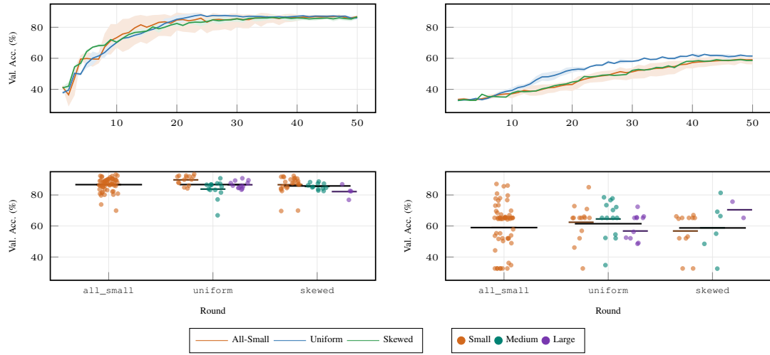
Fig. 8. FedMD tier-heterogeneity ablation on HomeOccupancy. Top: mean validation-accuracy curves over completed seeds (shaded bands: seed range), IID (left) and non-IID (right) on a shared y-axis. Bottom: per-client final accuracy (mean of the last five rounds, seeds pooled). Each distribution column is subdivided by architecture tier—small (orange), medium (teal), large (purple)—so tier counts are visible (e.g. skewed : 12/6/2); short coloured dashes mark tier means, the long black dash the column mean. Tier means differ by only a few points within every setting: under soft-label sharing, per-client accuracy is governed by the data partition, not by model capacity.
