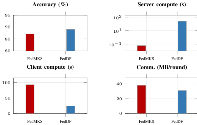
Fig. 10. Compute, communication, and accuracy comparison of FedMKS and FedDF on HomeOccupancy (cf. Table VII). FedMKS eliminates the server bottleneck at \approx 22\% higher communication and higher per-client compute.
