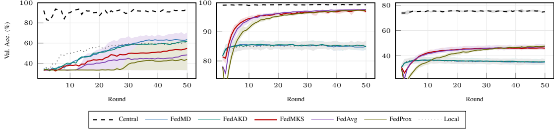
Fig. 3. Validation accuracy over 50 rounds under non-IID partitioning (Dirichlet \alpha=0.5 ). Panels: HomeOccupancy, MNIST, CIFAR-10. Curves show the mean over completed seeds; shaded bands show the seed range. FedAvg/FedProx use the all-small architecture.
