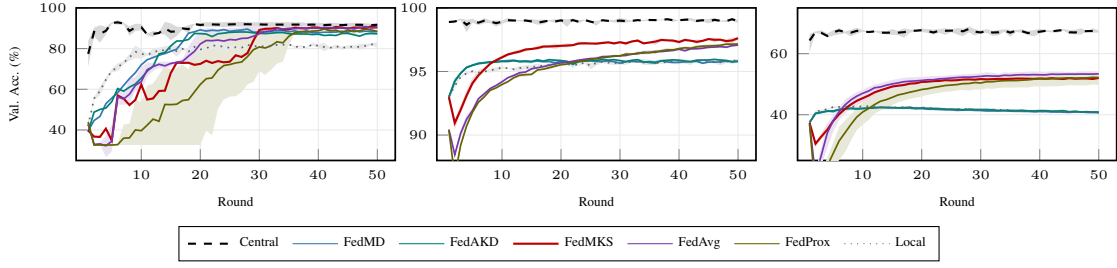
Fig. 2. Validation accuracy over 50 rounds under IID partitioning. Panels: HomeOccupancy, MNIST, CIFAR-10. Curves show the mean over completed seeds (up to three); shaded bands show the seed range. FedAvg/FedProx use the all-small architecture.
