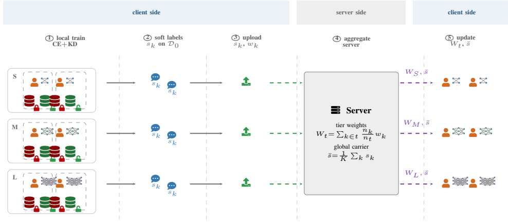
FedMKS: soft labels computed on each client ; the server averages intra-tier weights.
