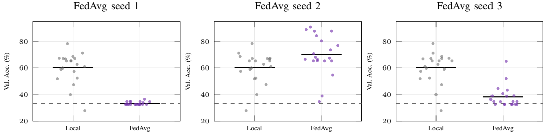
Fig. 5. HomeOccupancy non-IID, per-client final accuracy by seed (each client’s model evaluated after its local update). Grey dots (identical in every panel) are the Local-only clients; purple dots are FedAvg clients in seeds 1–3. In seeds 1 and 3 every FedAvg client sits at chance (33.3%)—the shared model collapses collectively—while seed 2 retains a healthy spread comparable to Local.
