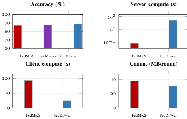
Fig. 10. Compute, communication, and accuracy comparison of FedMKS and FedDF-var on HomeOccupancy (cf. Table VII). FedMKS eliminates the server bottleneck at \approx 22\% higher communication and higher per-client compute.
