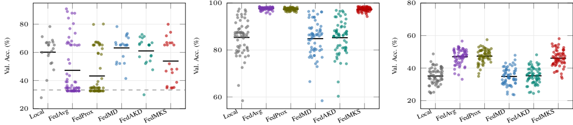
Fig. 4. Per-client final validation accuracy (mean of the last five rounds, evaluated on each client’s model after its local update) under non-IID partitioning. Each dot is one client; all completed seeds are pooled (60 dots per three-seed method, 20 per single-seed method). Black dashes mark method means; the grey dashed line marks chance level (33.3% for HomeOccupancy, 10% for CIFAR-10). Left: HomeOccupancy—in the two collapsed FedAvg/FedProx seeds all clients sit at chance, while KD-based and local clients spread around \approx 60\% . Middle/right: MNIST and CIFAR-10—no client collapses; weight sharing lifts every client above the local mean.
