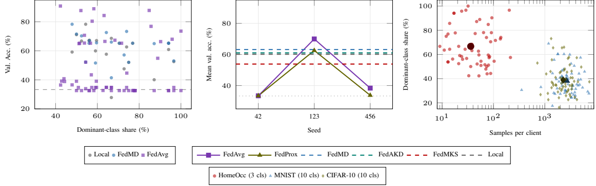
Fig. 6. Data distribution decides whether weight averaging survives. (a) HomeOccupancy non-IID: per-client final accuracy vs. each client’s dominant-class share. FedAvg clients in the two collapsed seeds sit at chance at every share, including nearly balanced ones—collapse is a property of the averaged model, not of any client’s data. Per-client models (Local, FedMD) never collapse; their degradation with share is quantified in Fig. 7. (b) Mean accuracy per seed: FedAvg and FedProx collapse in two of three seeds while the KD-based methods and Local (single seed, dashed references) hold \approx 54 –63%; FedMKS never falls below 53%, so its worst case exceeds the weight-sharing worst case by \approx 20 points. (c) Per-client partitions of all benchmarks in the (samples, dominant-share) plane (all seeds pooled; large marks are dataset means). HomeOccupancy alone occupies the high-skew/low-data corner.
