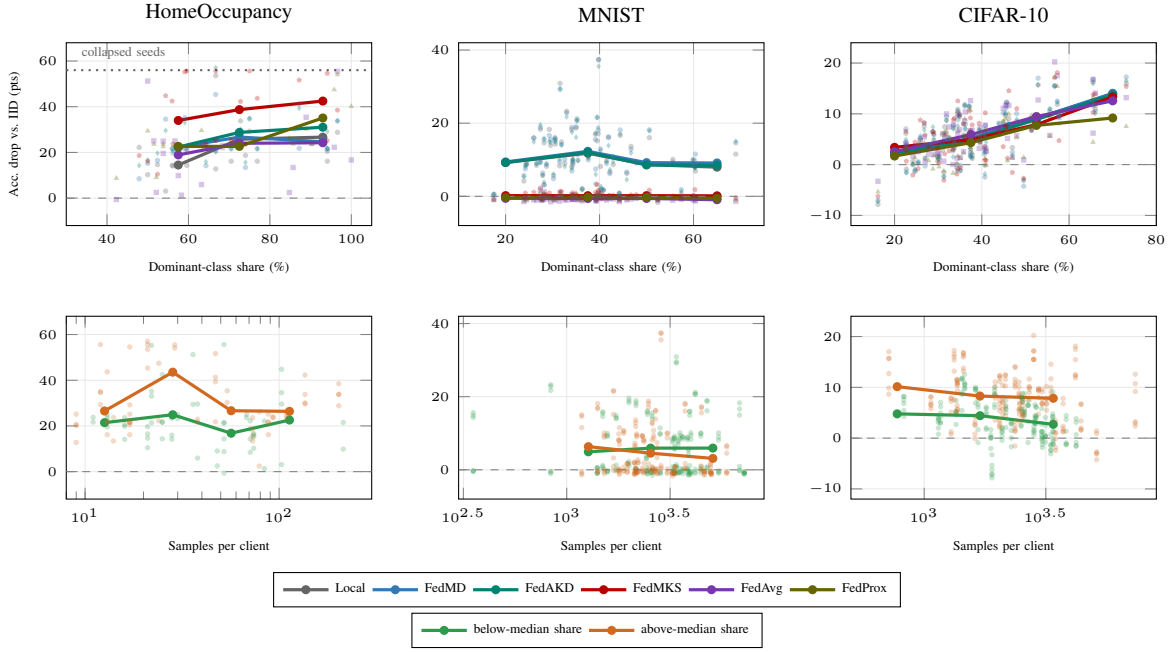
Fig. 7. Per-client accuracy decline under non-IID, measured as the drop from each method’s own IID mean (dots: individual clients, seeds pooled; thick lines: binned means). Top: decline vs. dominant-class share, per method. (a) HomeOccupancy: the drop grows with share for every method that keeps per-client models ( r=+0.73 for FedProx’s surviving seed), while the two collapsed FedAvg/FedProx seeds form a flat band at \approx 56 points (dotted)—their bias is total and independent of the partition. (b) MNIST: weight sharing loses essentially nothing; only local-model methods drop \approx 9 points. (c) CIFAR-10: the share–decline link is the strongest of any benchmark ( r \approx +0.6 ). Bottom: the same decline vs. samples per client, pooled over methods and split at each dataset’s median share. On HomeOccupancy (d) more data does not rescue the above-median half (extra samples are mostly more of the dominant class); on MNIST (e) drops are negligible at every size; on CIFAR-10 (f) larger partitions reduce the drop for both halves—size helps only where samples are already plentiful.
