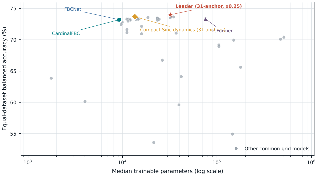
Accuracy-efficiency landscape across all 43 common-recipe models
