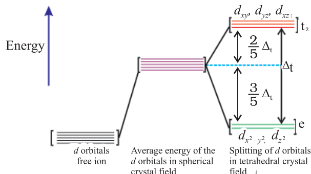
Fig.5.9: d orbital splitting in a tetrahedral crystal field.
