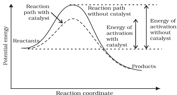
Fig. 3.11: Effect of catalyst on activation energy
