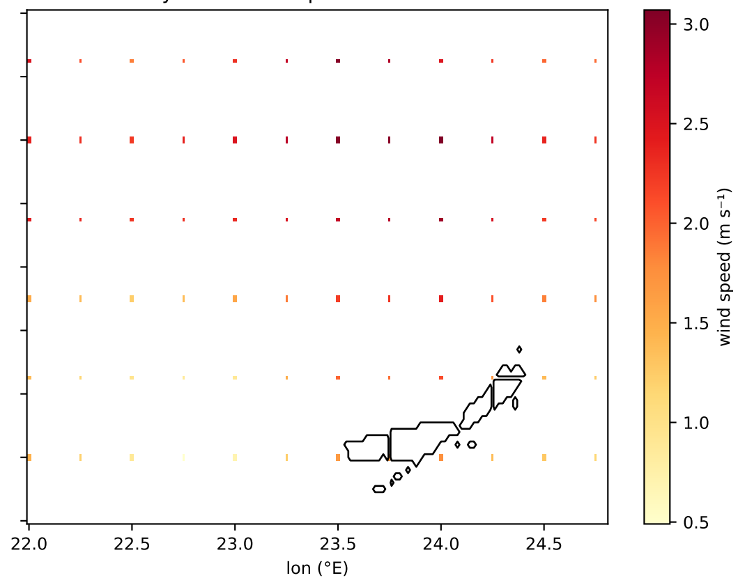
ERA5 daily mean wind speed + SST-mask contour
