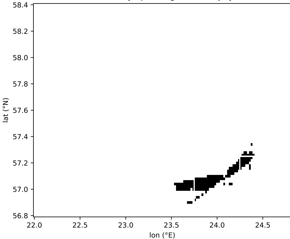
CS1 — SST-only upwelling mask, 16 July 2021
