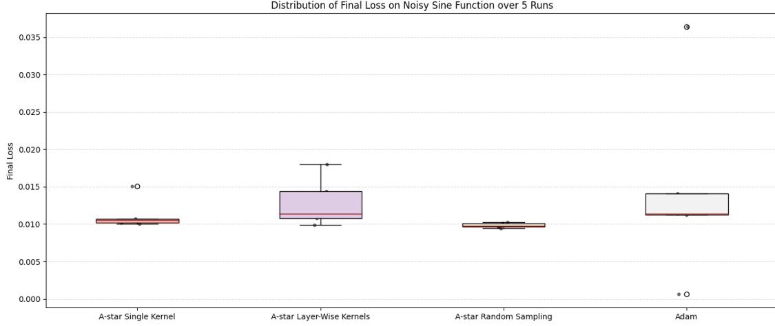
Figure 9.11: Distribution of Final Loss for Small Net.
