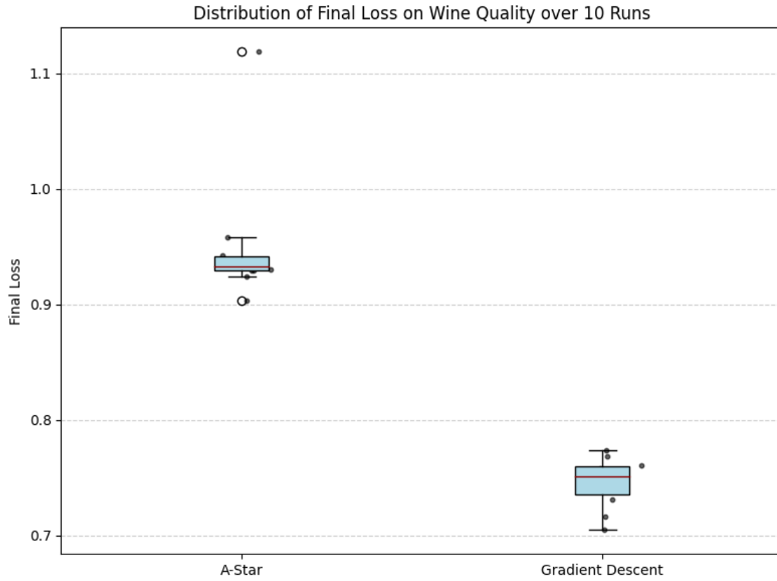
Figure 4.17: Final Loss Box Plot for I_{\max} = 2,000 Iterations.
