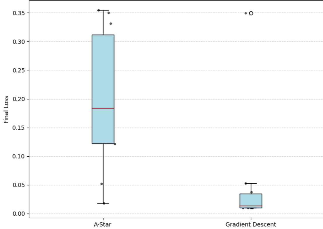
Figure 4.9: Final Loss Box Plot for I_{\max} = 2,000 Iterations.
