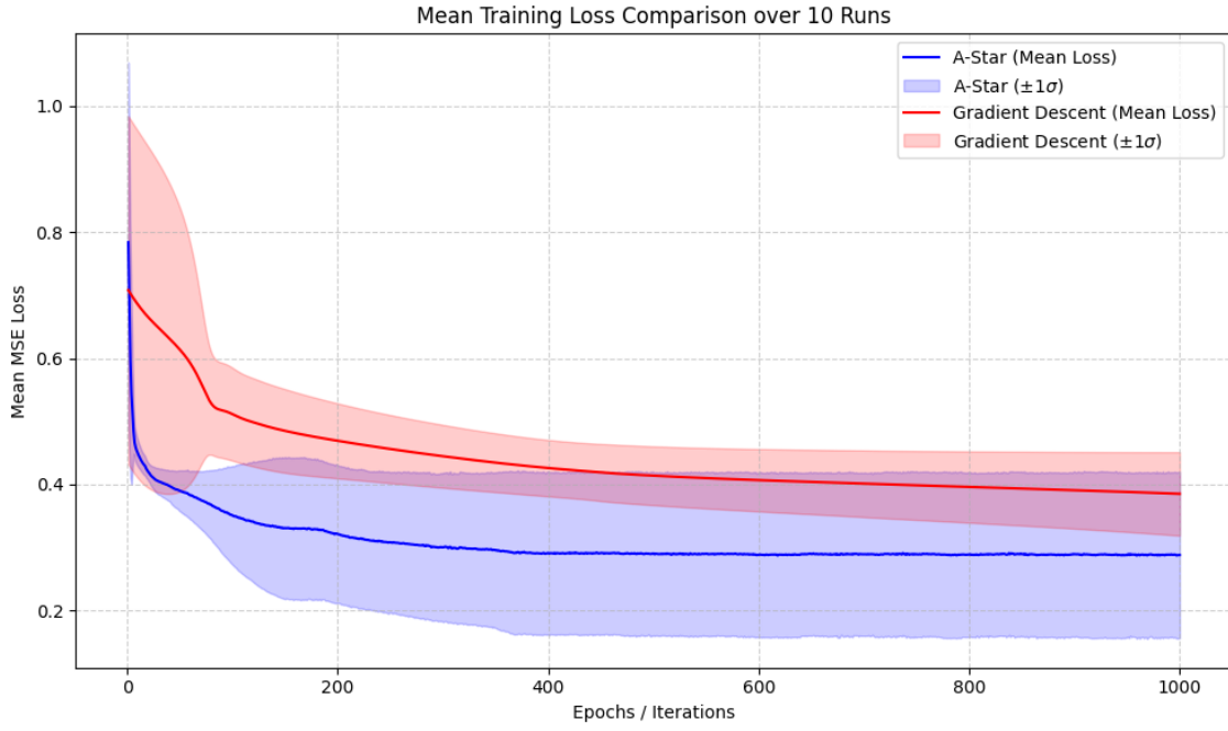
Figure 4.7: Mean Loss Trajectory with Standard Deviation Shading for I_{\max} = 1,000 Iterations. This plot illustrates the average loss over ten independent runs for both A* Search (Novel) and Gradient Descent (Classic), with the shaded region representing \pm 1 standard deviation. It highlights convergence speed and the consistency of each algorithm's performance over time.
