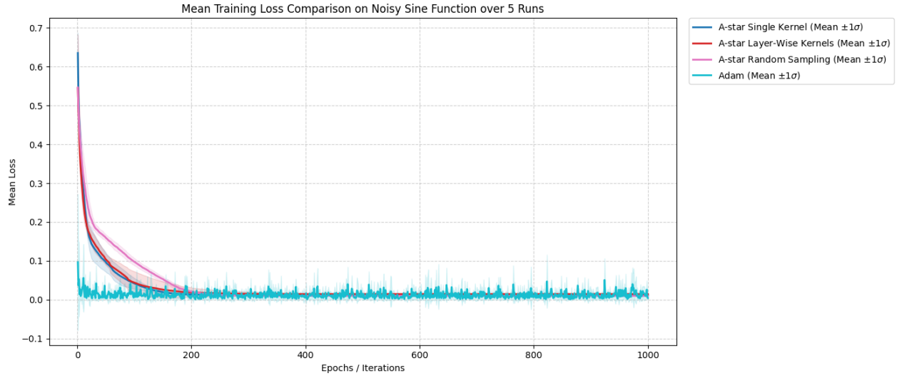
Figure 9.13: Medium Net convergence: A^* strategies vs. Adam on Noisy Sine.
