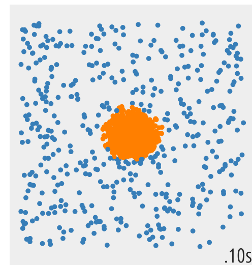
Isolation Forest
