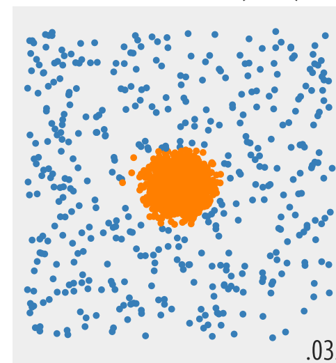
One-Class SVM (SGD)
