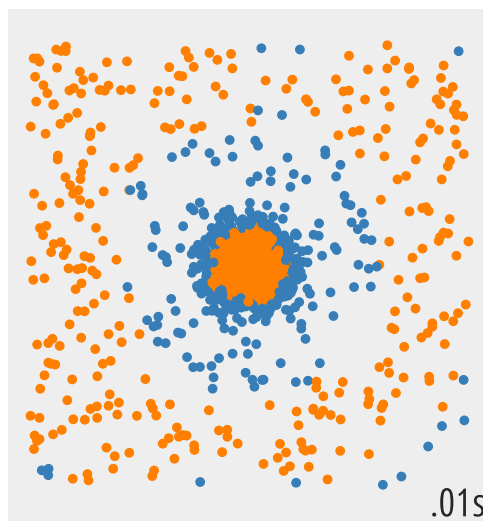
Local Outlier Factor
