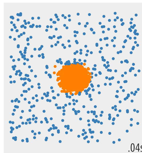
One-Class SVM
