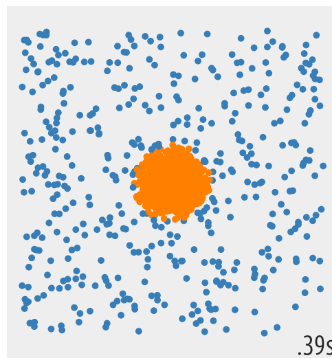
Robust covariance
