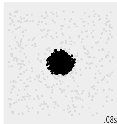
Isolation Forest
