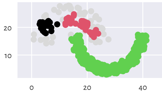
HDBSCAN (min_cluster_size=12)
