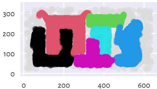
(min_cluster_size=50, min_samples=5)
