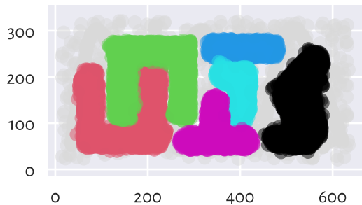
(min_cluster_size=10, min_samples=50)
