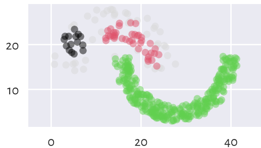
HDBSCAN (min_cluster_size=10)
