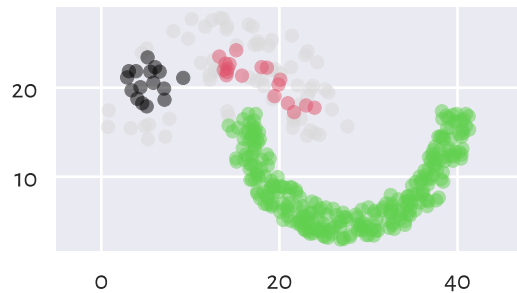
HDBSCAN (min_cluster_size=14)
