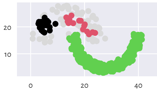
HDBSCAN (min_cluster_size=14)
