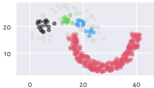
HDBSCAN (min_cluster_size=11)
