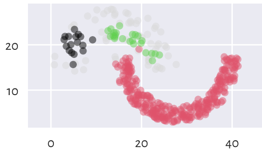
HDBSCAN (min_cluster_size=13)
