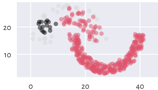
HDBSCAN (min_cluster_size=15)
