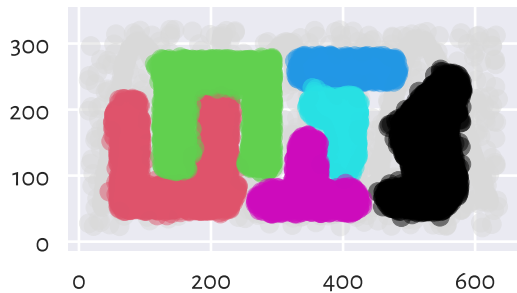
(min_cluster_size=50, min_samples=50)
