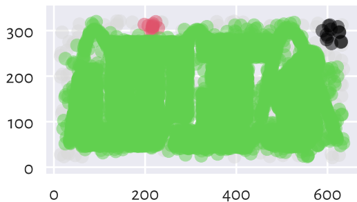
(min_cluster_size=5, min_samples=5)
