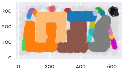
(min_cluster_size=10, min_samples=5)
