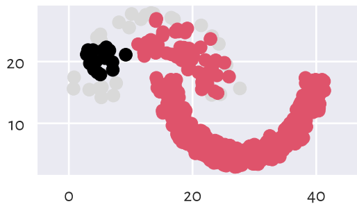
HDBSCAN (min_cluster_size=15)
