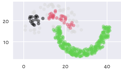
HDBSCAN (min_cluster_size=12)
