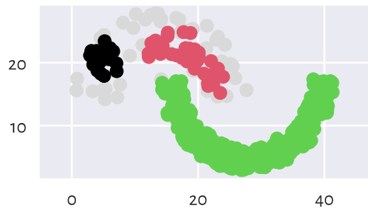
HDBSCAN (min_cluster_size=10)
