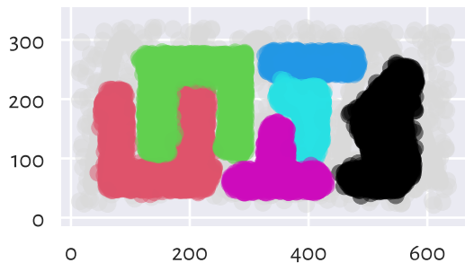
(min_cluster_size=5, min_samples=50)
