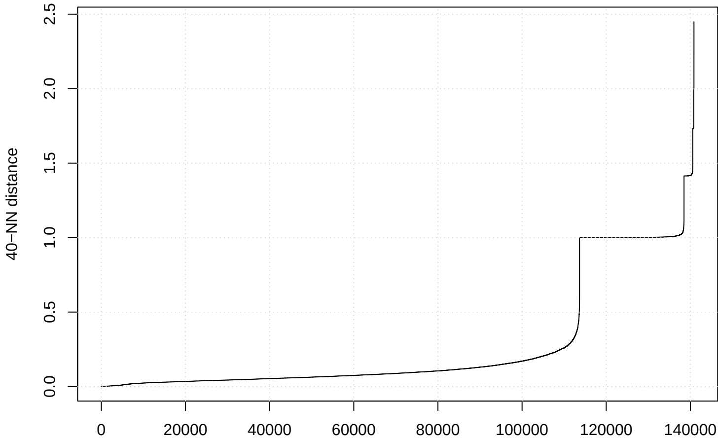
K-Distance Plot (k = 40 )
