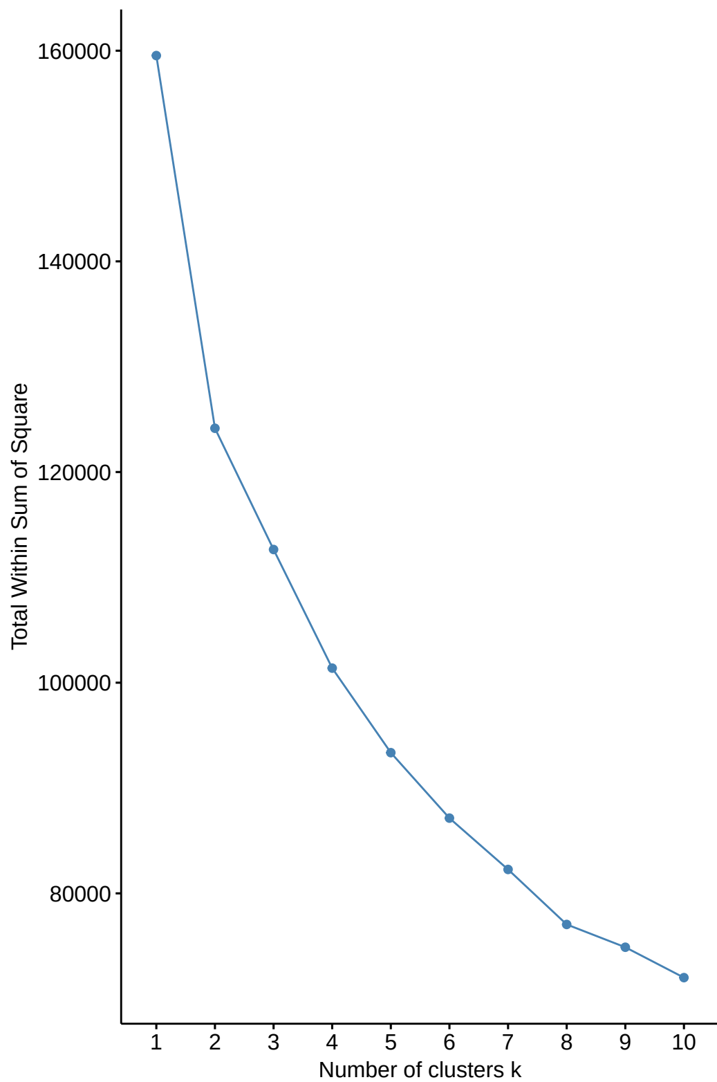
Elbow Method (Sampled)
